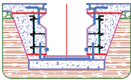
Double skin for bad ground conditions
