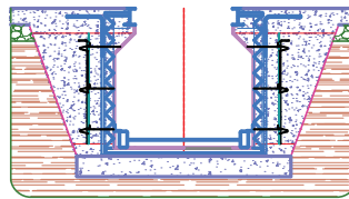
Double skin for bad ground conditions
